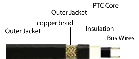
Structure of Model PSL/PSLL series-CR
