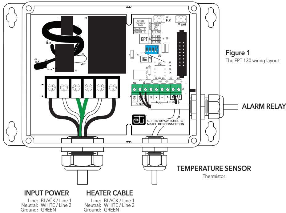
FIGURE 1. The FPT 130 wiring layout.
