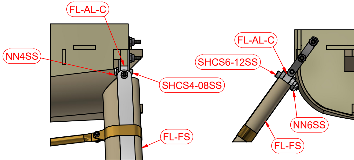
Pick-up #4 Scale 1/2
