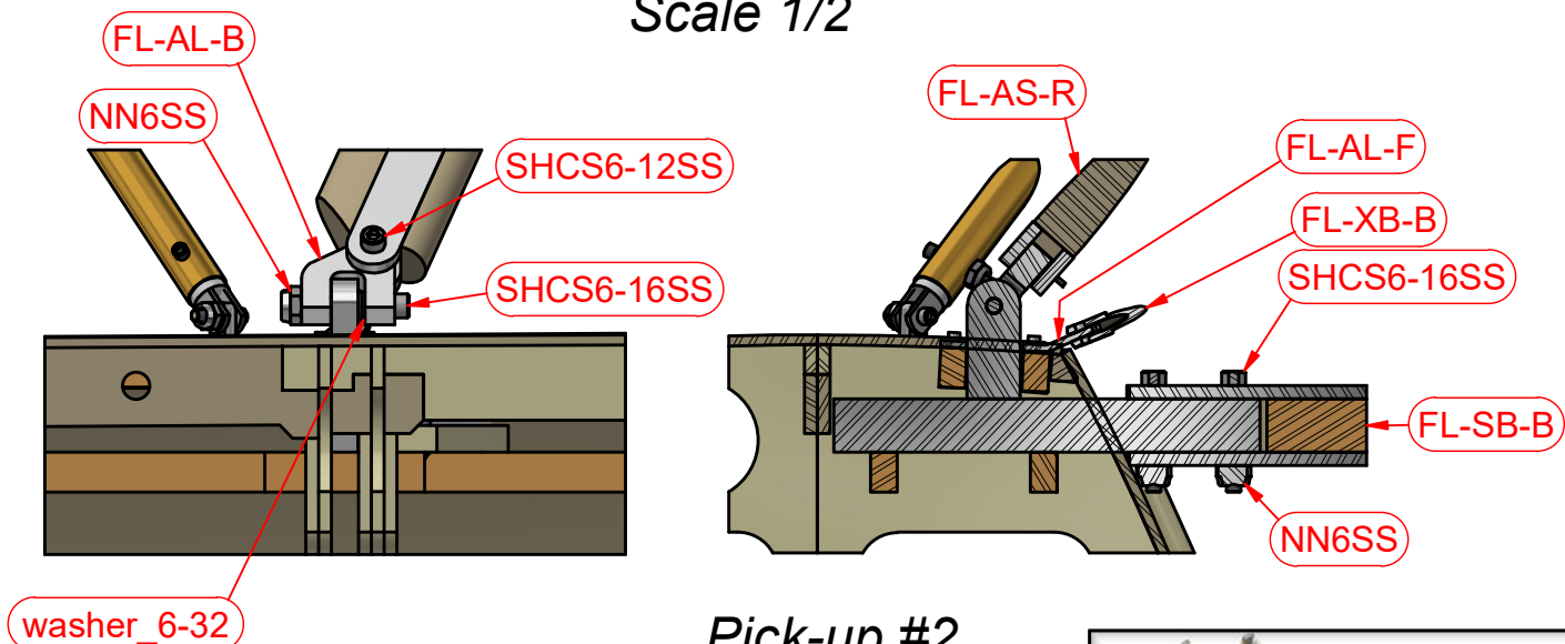
Pick-up #1 Scale 1/2
