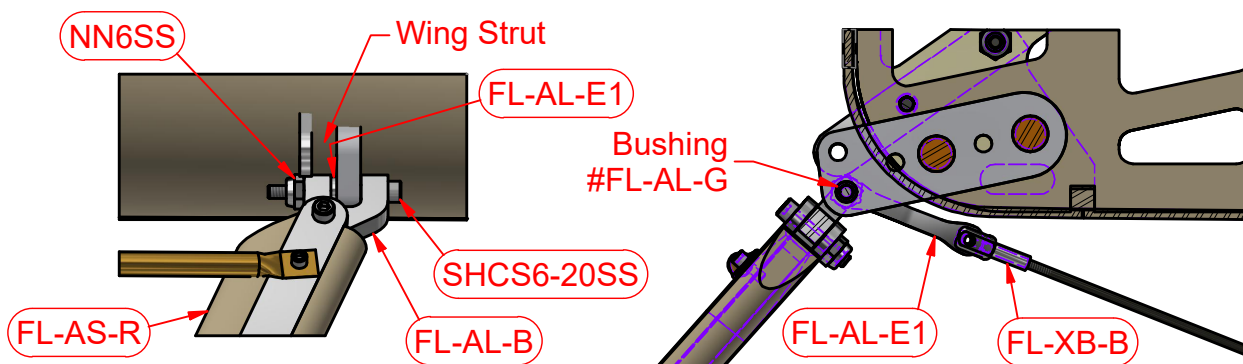
Pick-up #1 Scale 1/2
