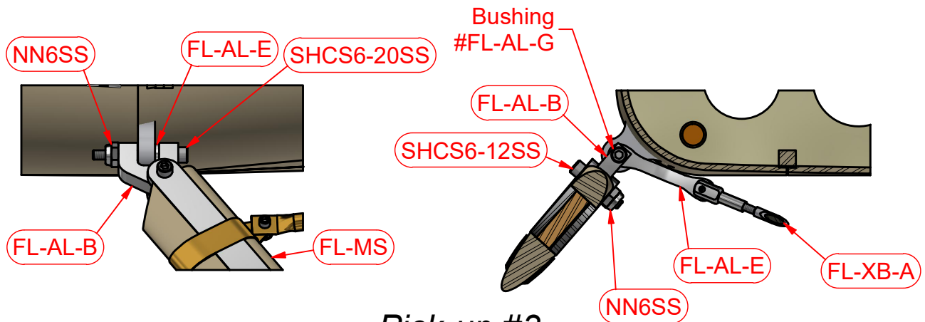
Pick-up #3 Scale 1/2
