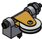
Pulley-A Pulley (7 req.)
