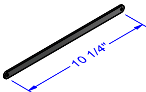
□ FL-FS-01 Aluminium 1/8" x 1/2" (4 req.)
