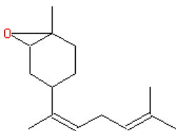
(xi) trans-Z-α-Bisabolene epoxide
