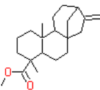
(xxiv) Kaur-16-en-18-oic acid, methyl ester,(4β)-
